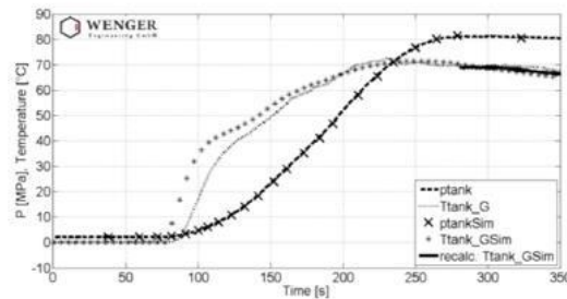
Figure 3 - Model validation [5] for protocol development for light duty vehicles in [2]
